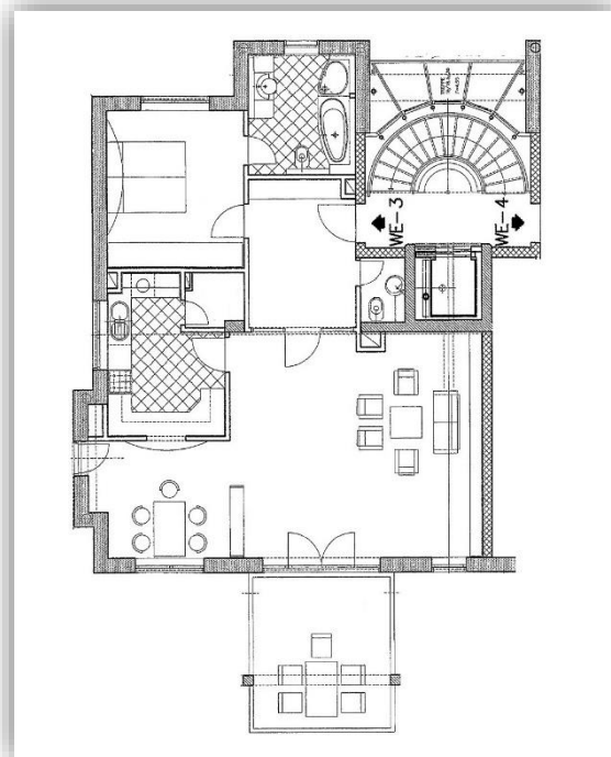
11: GRUNDRISS
